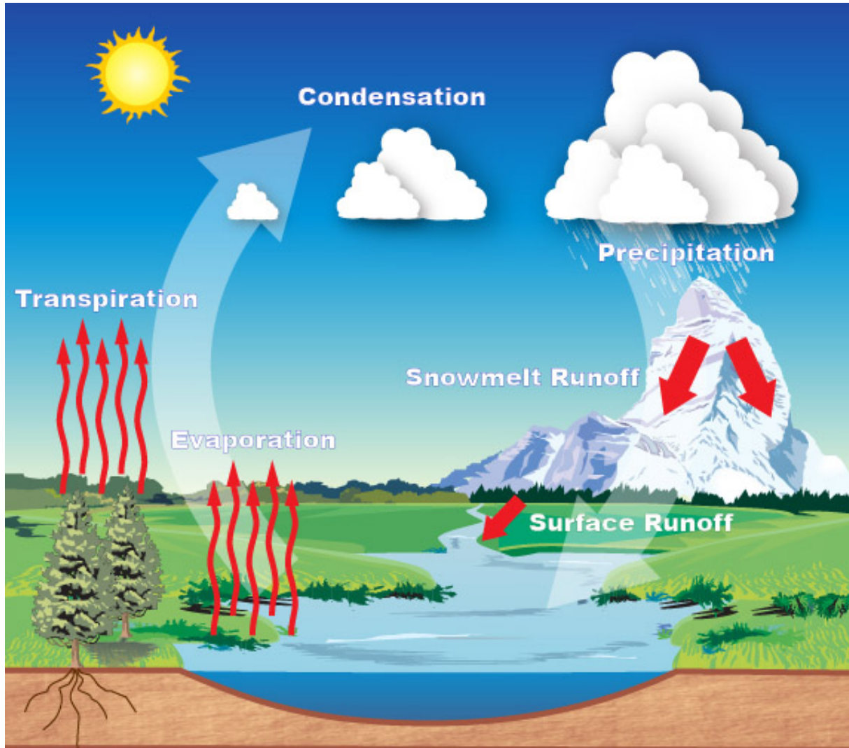
The basic hydrologic (water) cycle
